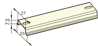
Mounting dimension of externally mounted handle
